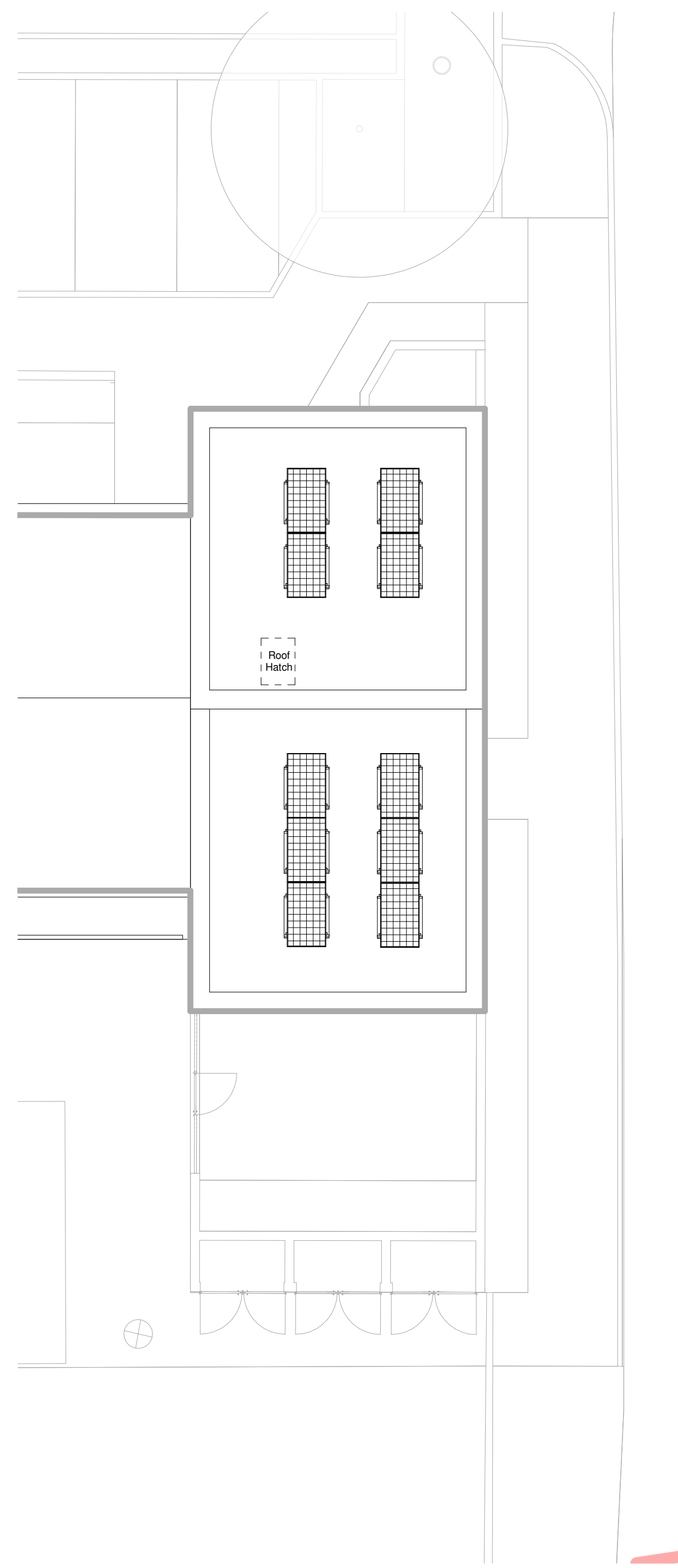
3 D_050 Block B - Roof Plan 1 : 100
