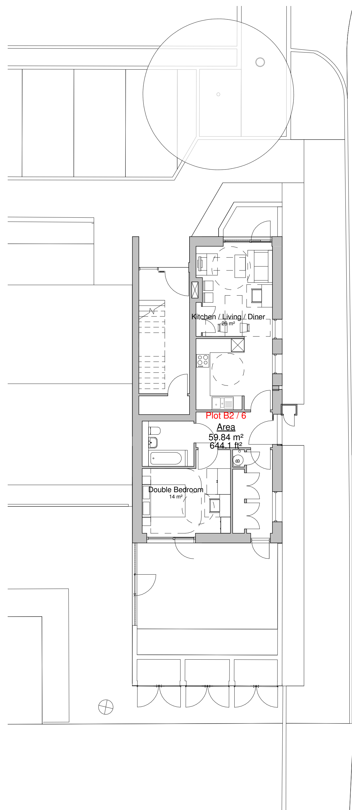
1 D_050 Block B - Ground Floor Plan 1 : 100
