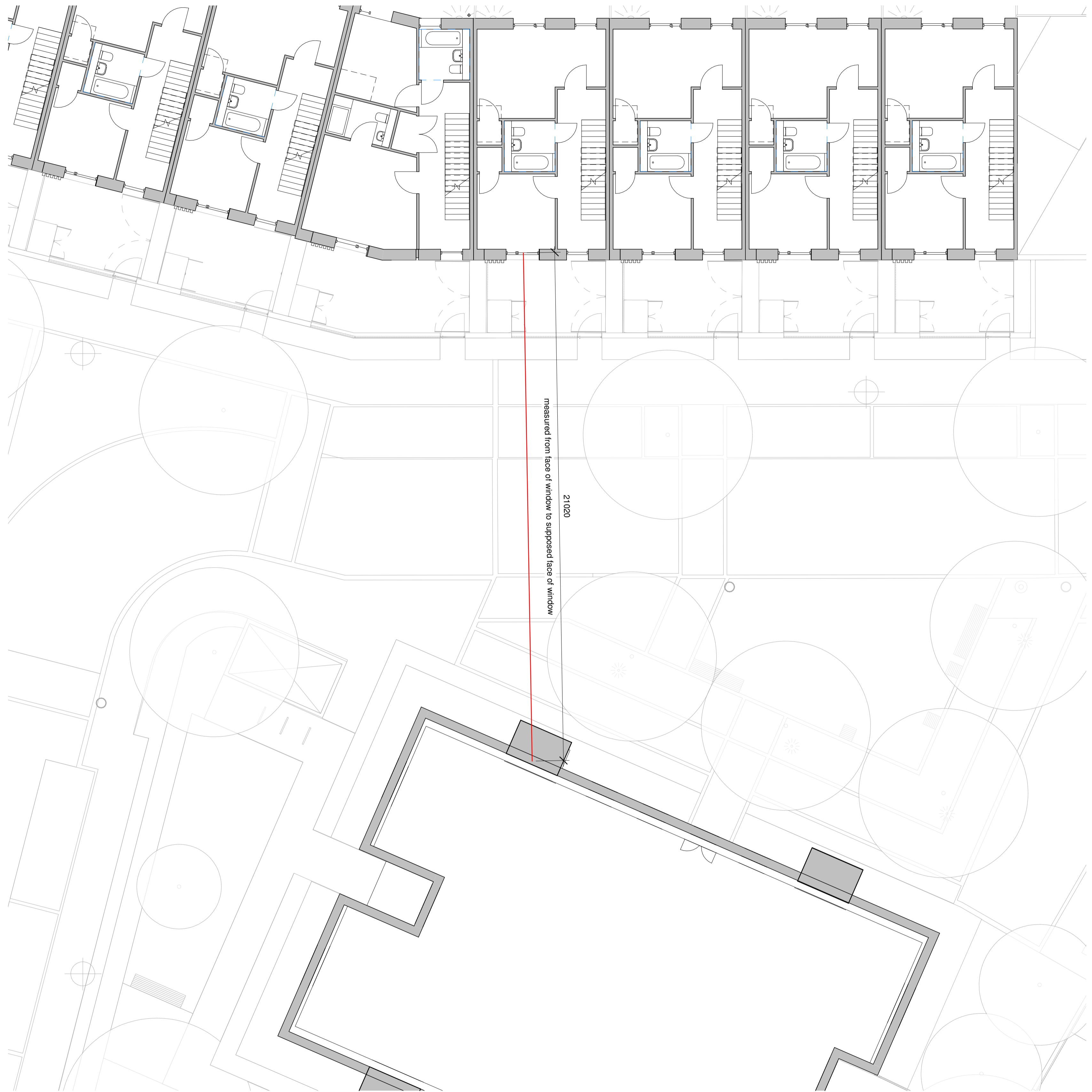
Plot 21 Privacy Distance - First Floor 1 : 100
